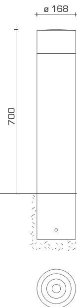
Borne \varnothing 168 PMR
