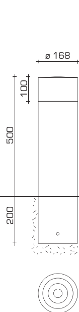
Borne \varnothing 168
